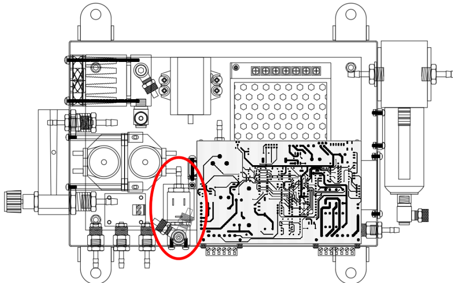
Figure 19, 3-way purge valve
