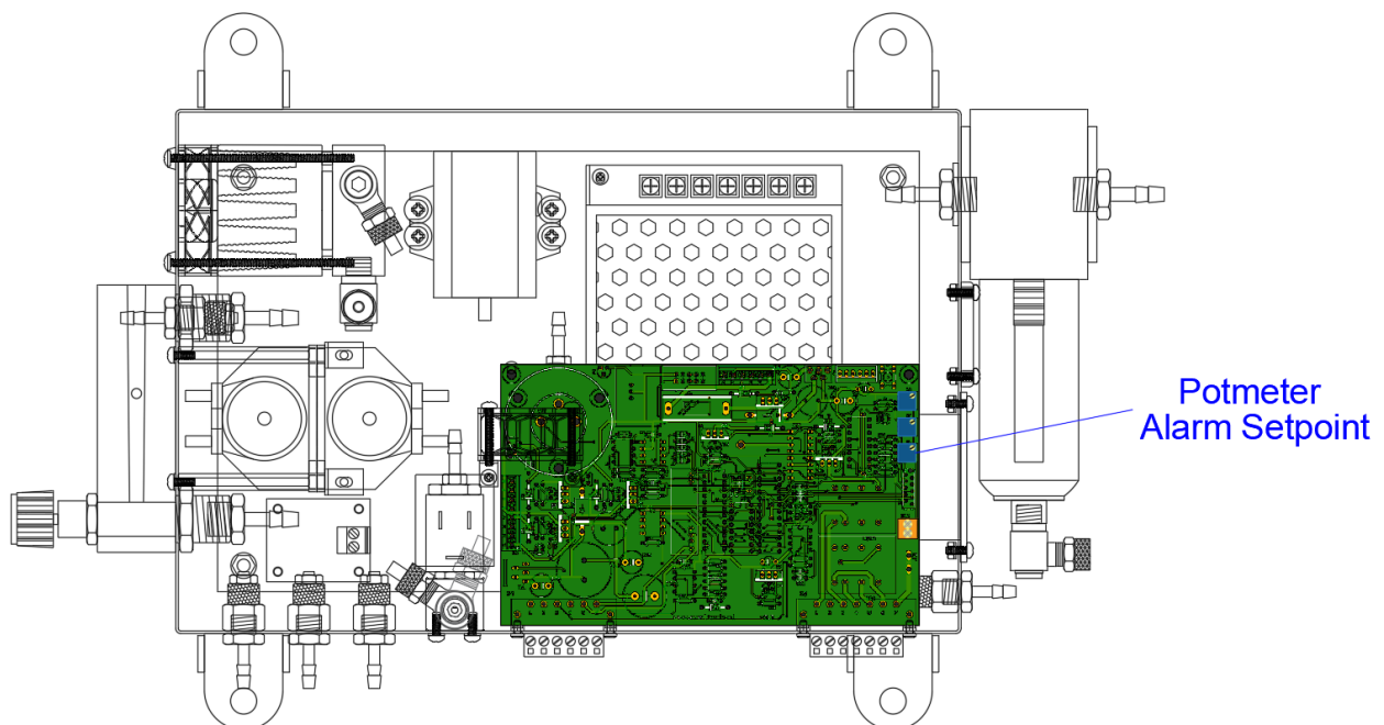
Figure 15, Potentiometer for the alarm limit for the CO measurement value
