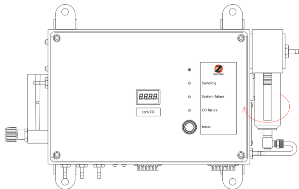
Figure 21, Sample filter
