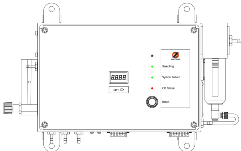
Figure 18, Status LEDs on front panel
