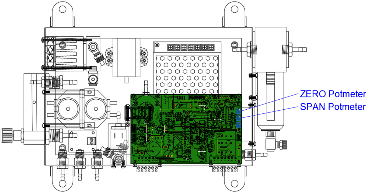
Figure 14, Zero and span potentiometers
