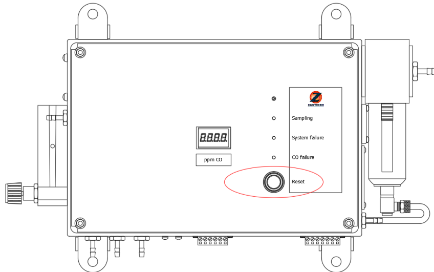
Figure 12, Reset switch
