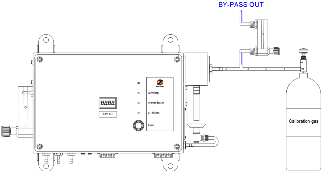
Figure 13, Calibration with calibration gas using a bypass
