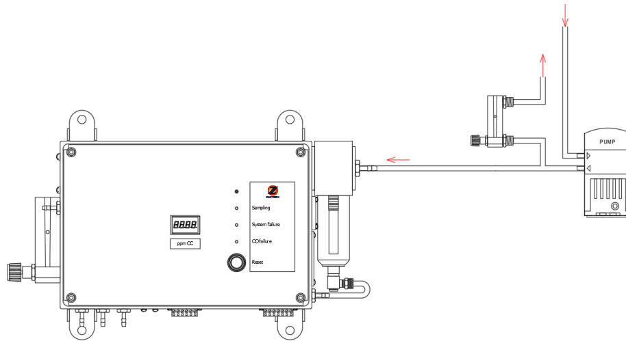
Figure 6, Connecting the bypass
