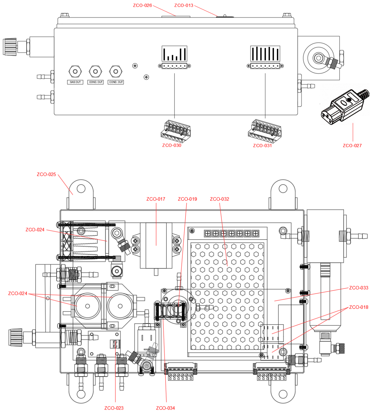
Figure 23, Various spare parts
