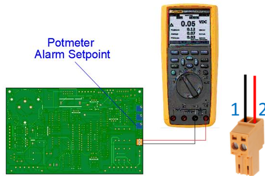
Figure 16, Configuring the alarm level
