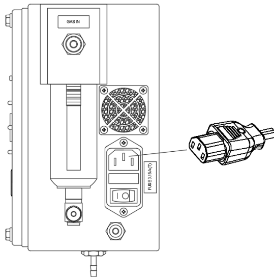
Figure 8, C13 connector
