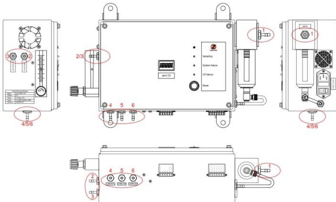
Figure 3 Various hose connections
