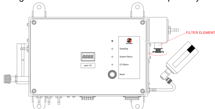
Figure 22, Removing the filter element
